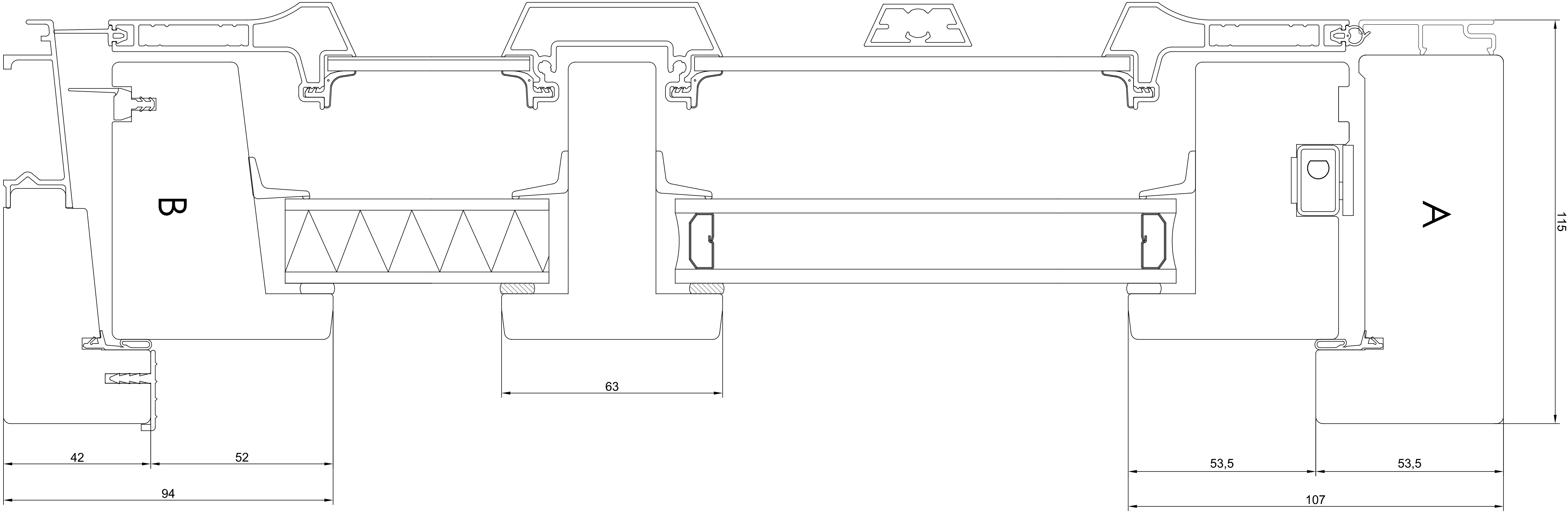
MAIN VERTICAL CROSS SECTION
