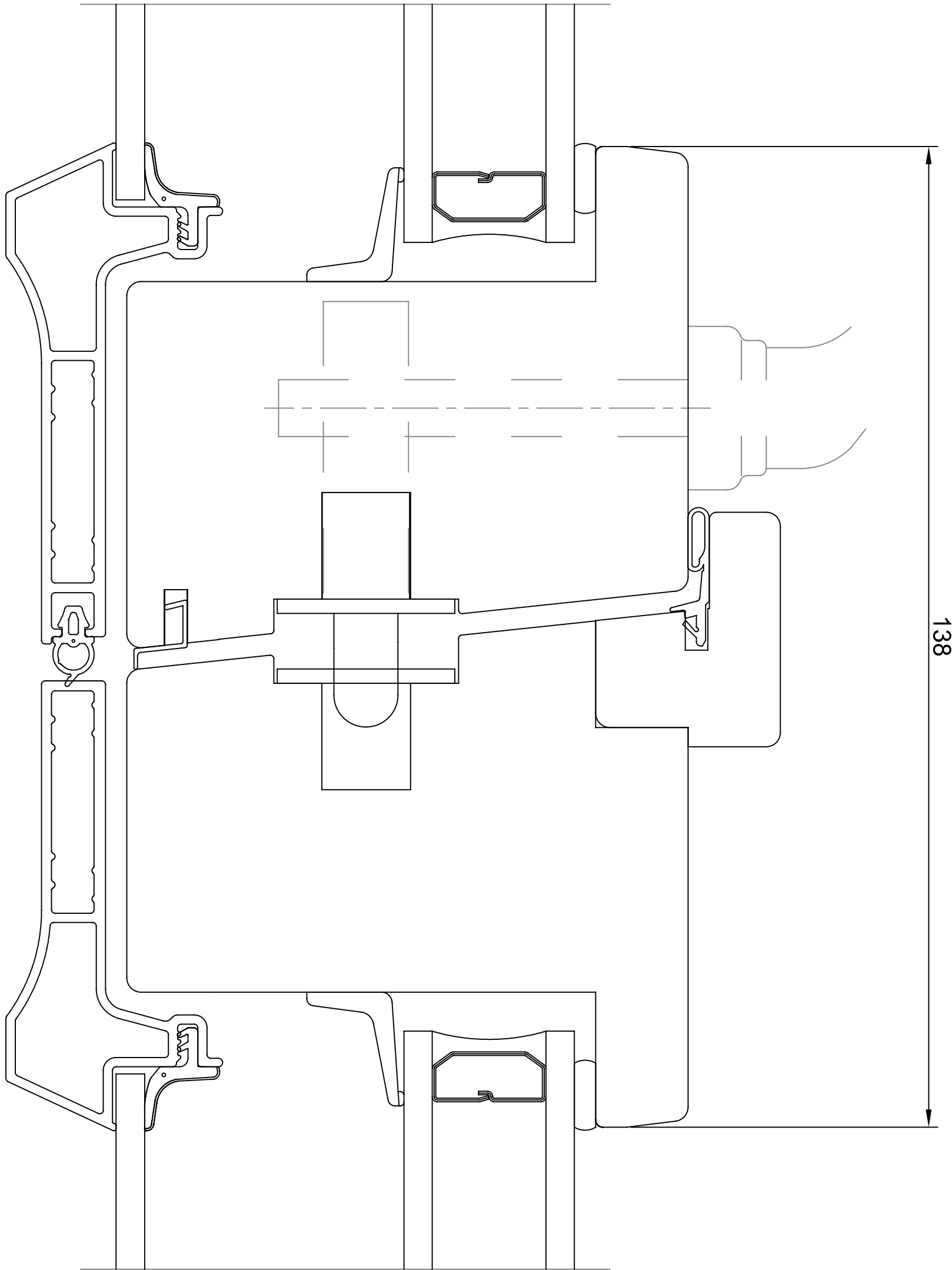
HORIZONTAL CS OPTION - Two horizontal abutting sashes.
