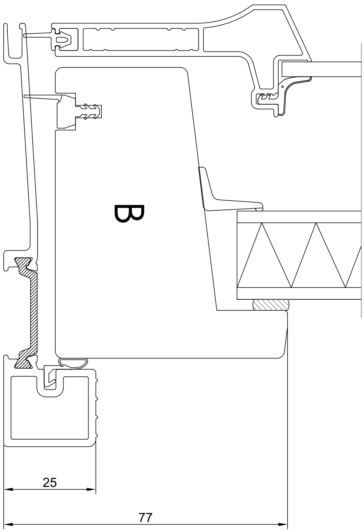
VERTICAL CS OPTION - Low threshold.
