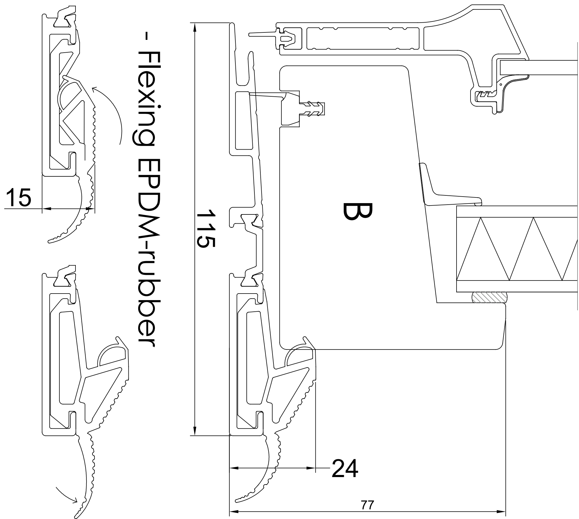
VERTICAL CS OPTION - Flex threshold.
