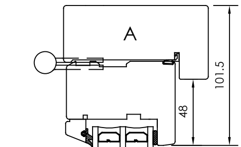
MAIN VERTICAL CROSS SECTION
