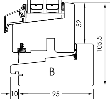
VERTICAL CS OPTION - Norwegian nose.
